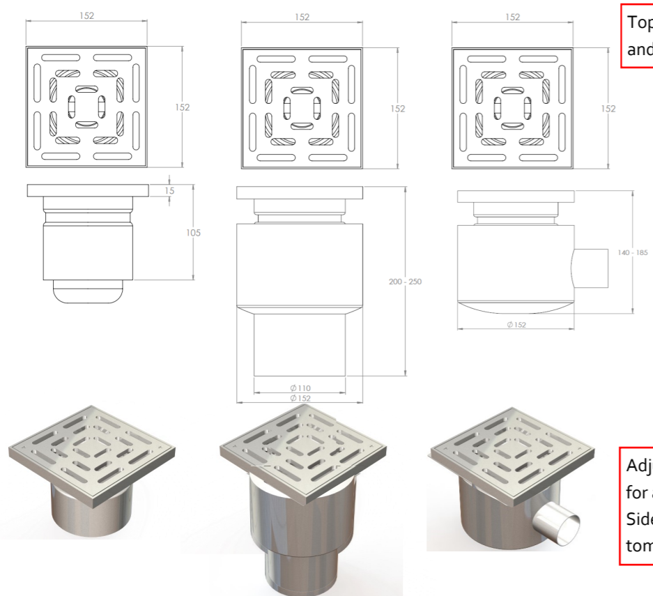
Top Part Only Adjustable Height Bottom Outlet (KVBO Body) Adjustable Height Side Outlet (KHBO Body)
