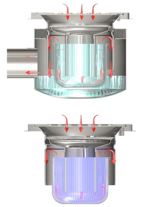
Waterflow for Adjustable Height Bodies
