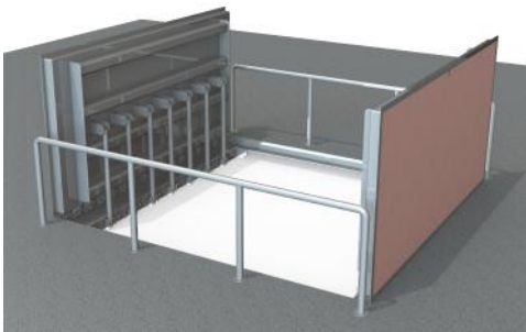
Optional Safety Barrier
